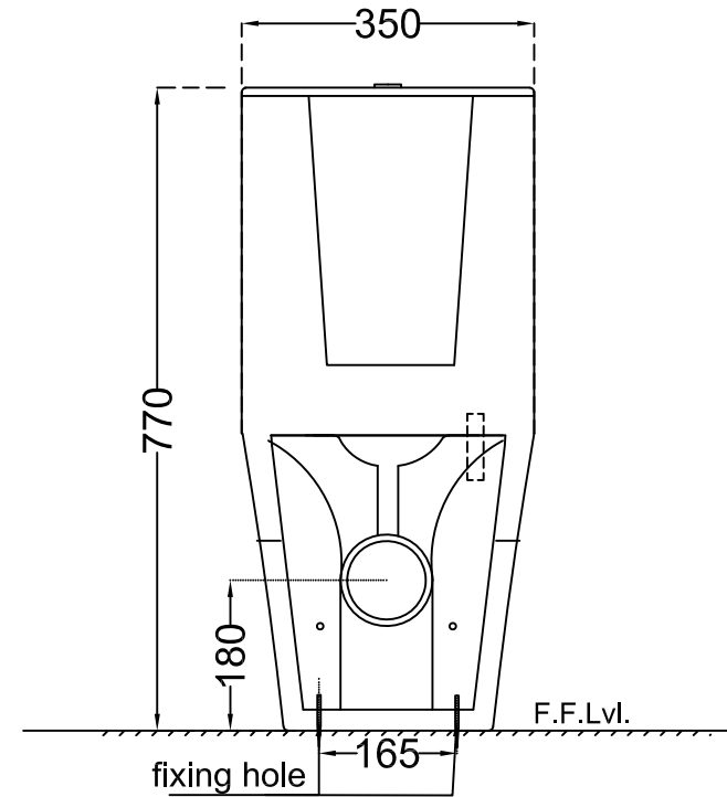
BACK VIEW
